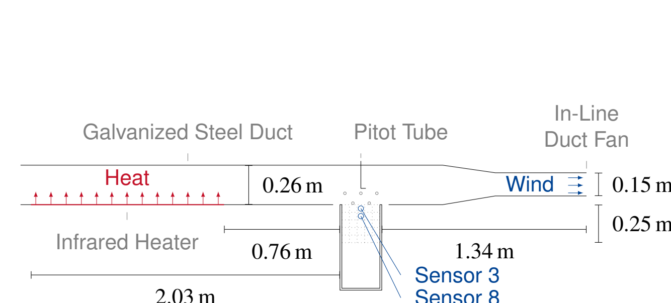
Figure 3: Setup for evaporation experiments performed by [2].
