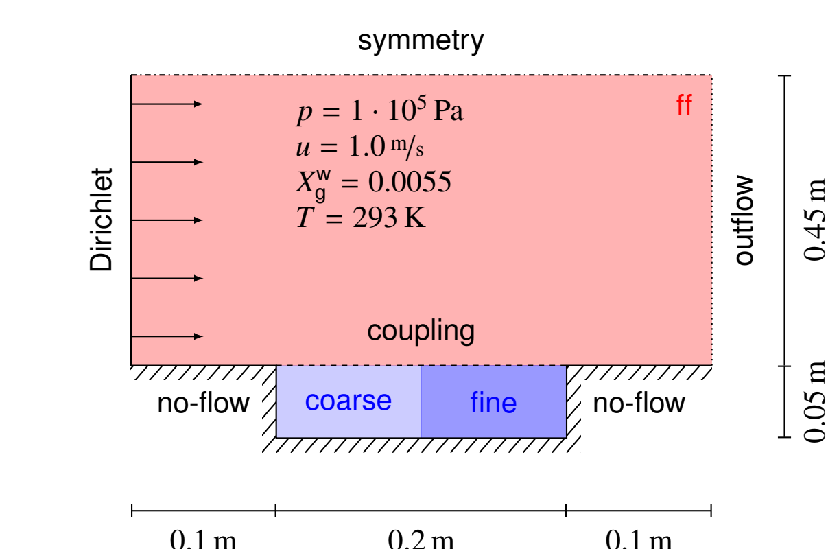
Figure 5: Simulation setup for evaporation from soil with a heterogeneity.
