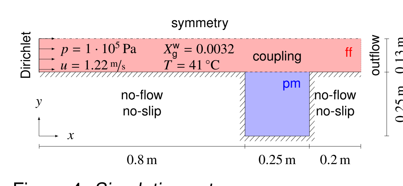
Figure 4: Simulation setup.
